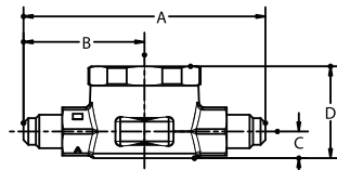
TYPE "MM" MALE FLARE X MALE FLARE
